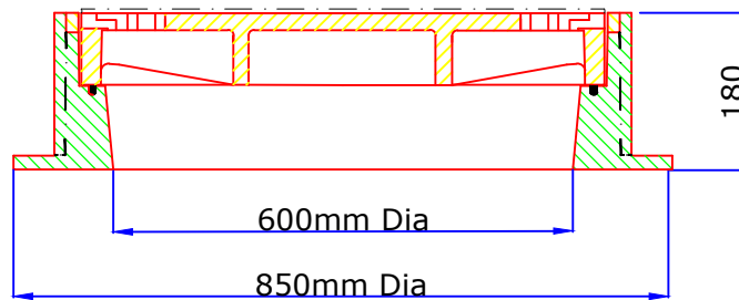
Sectional View
