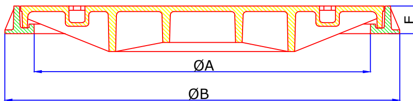
SECTIONAL VIEW
