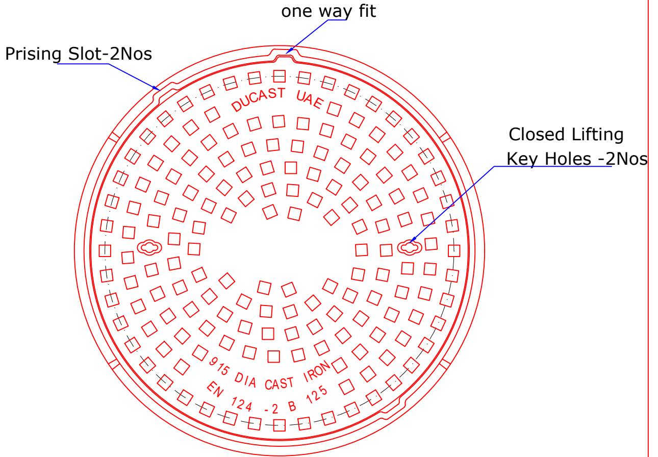
PLAN OF COVER & FRAME
