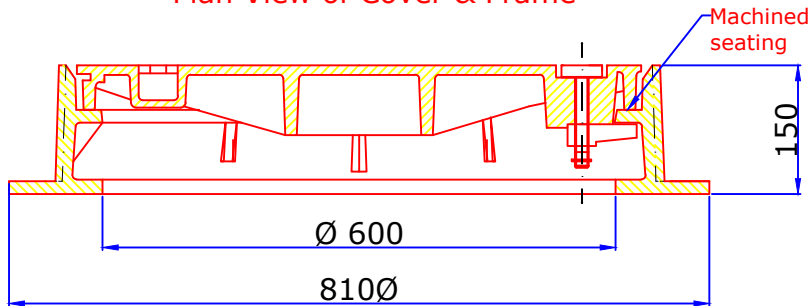
Sectional View of Cover & Frame @ M-M
