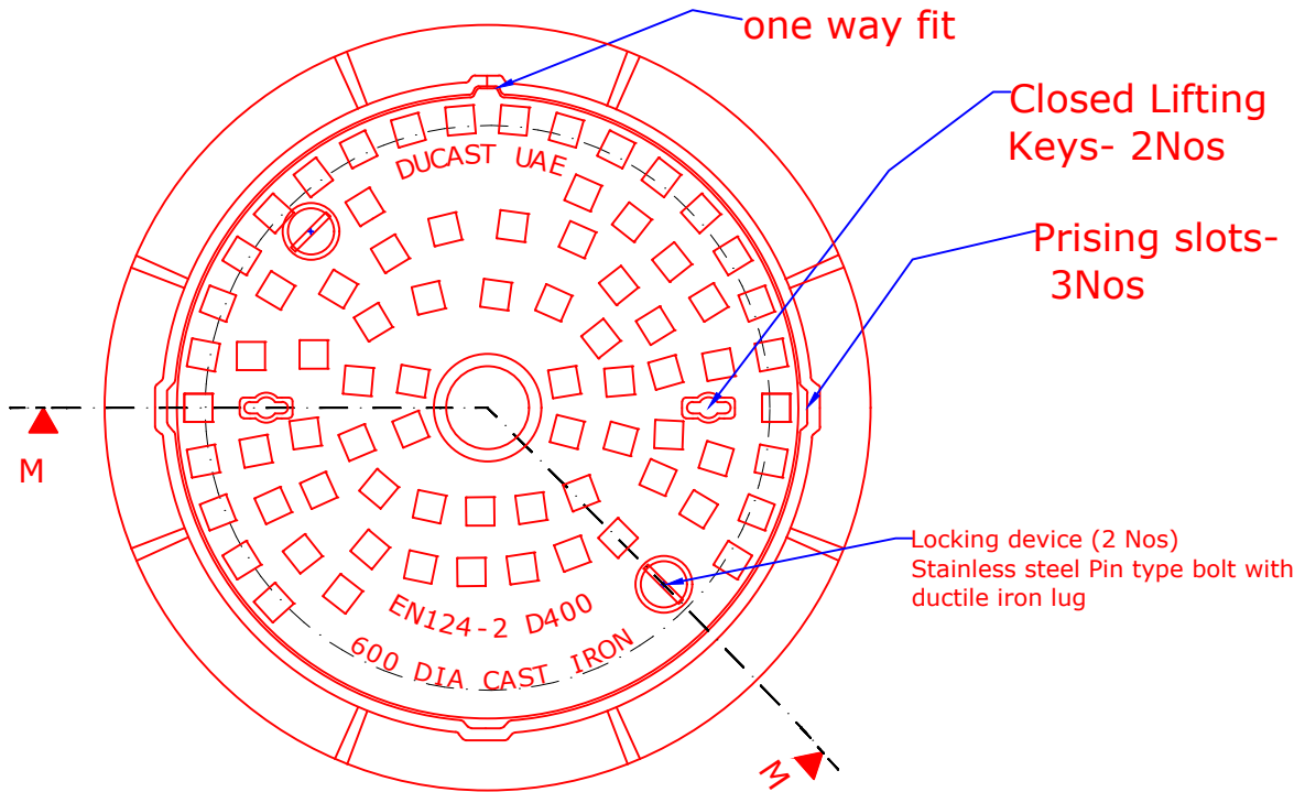
Plan View of Cover & Frame
