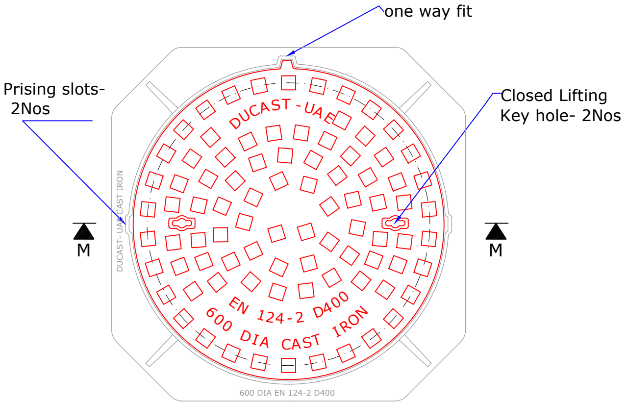
PLAN VIEW OF COVER & FRAME
