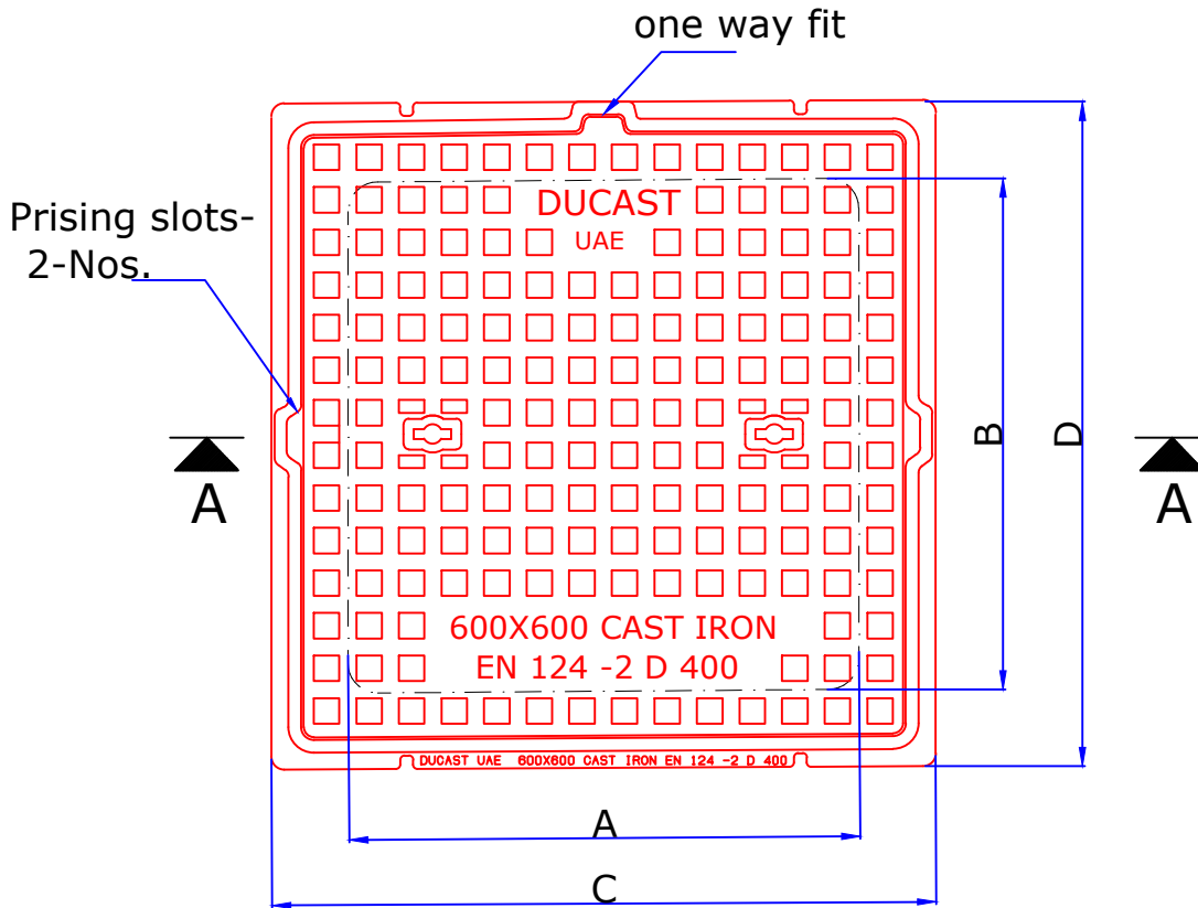
Plan View of Cover & Frame
