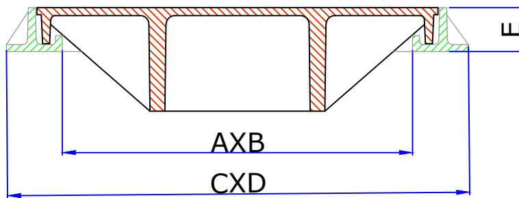
SECTIONAL VIEW
