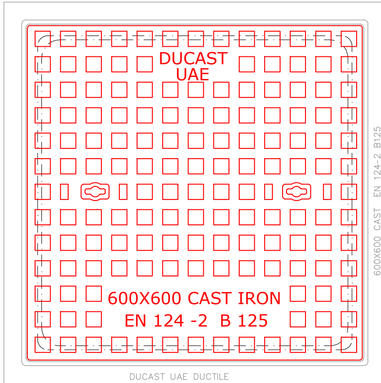
PLAN OF COVER & FRAME
