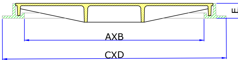
SECTIONAL VIEW
