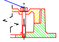
Sectional View at Bolting Area DETAIL- M
