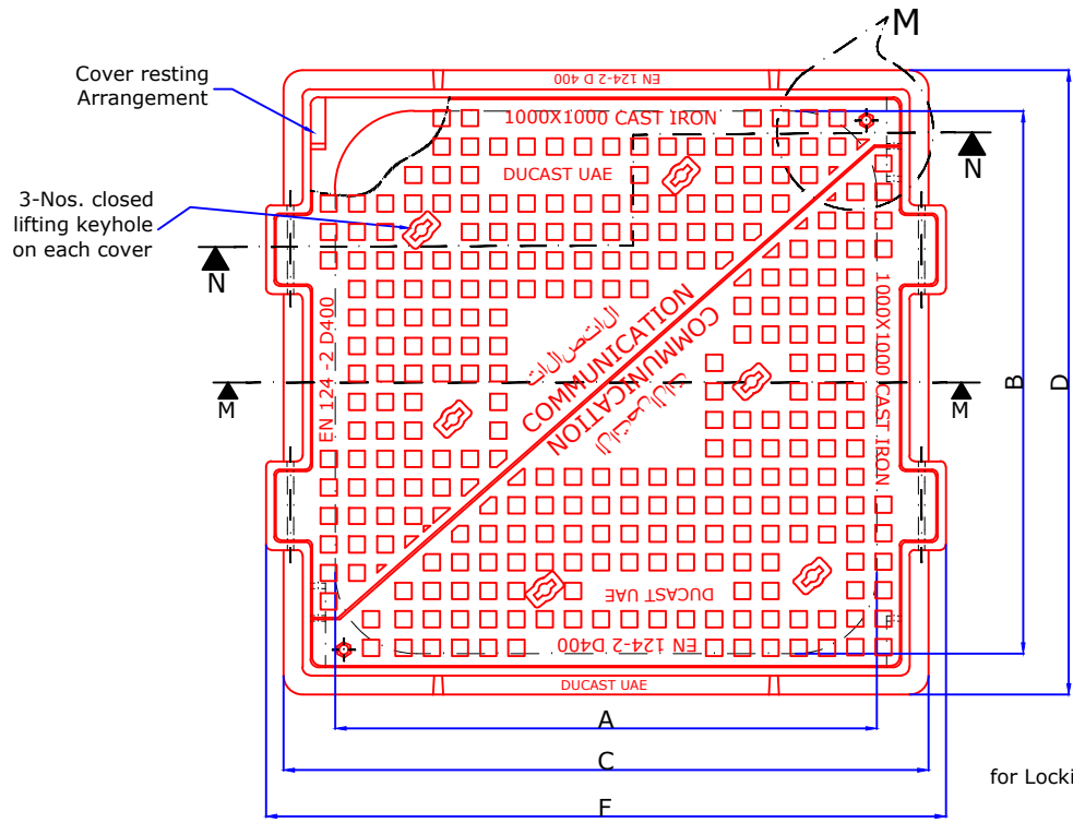
Plan of Cover & Frame
