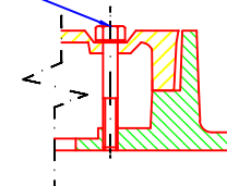
Sectional View at Bolting Area DETAIL- M
