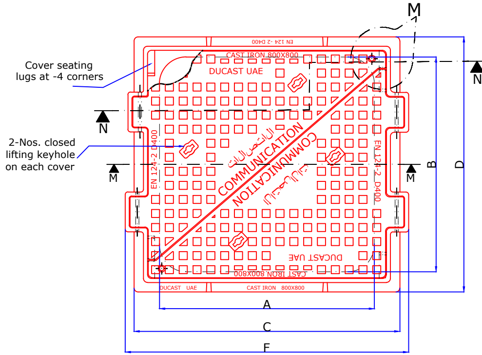
Plan of Cover & Frame
