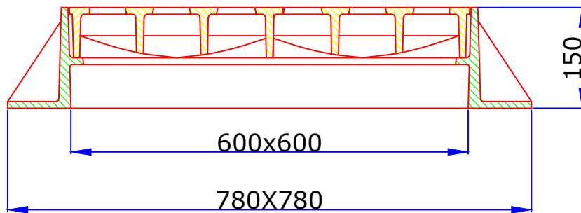
Sectional View of Grating & Frame @A-A
