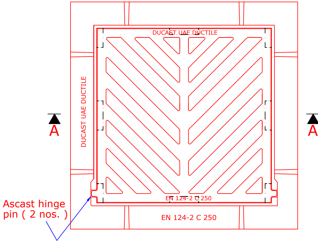
Plan View of Grating & Frame
