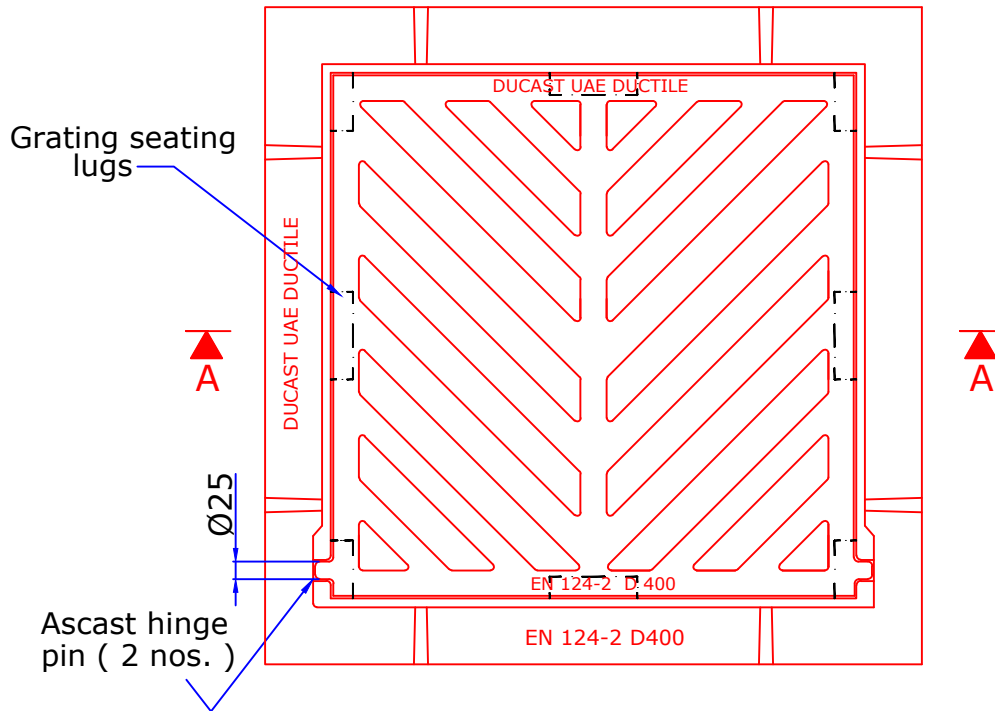
Plan View of Grating & Frame
