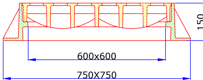
Sectional View of Grating & Frame @A-A
