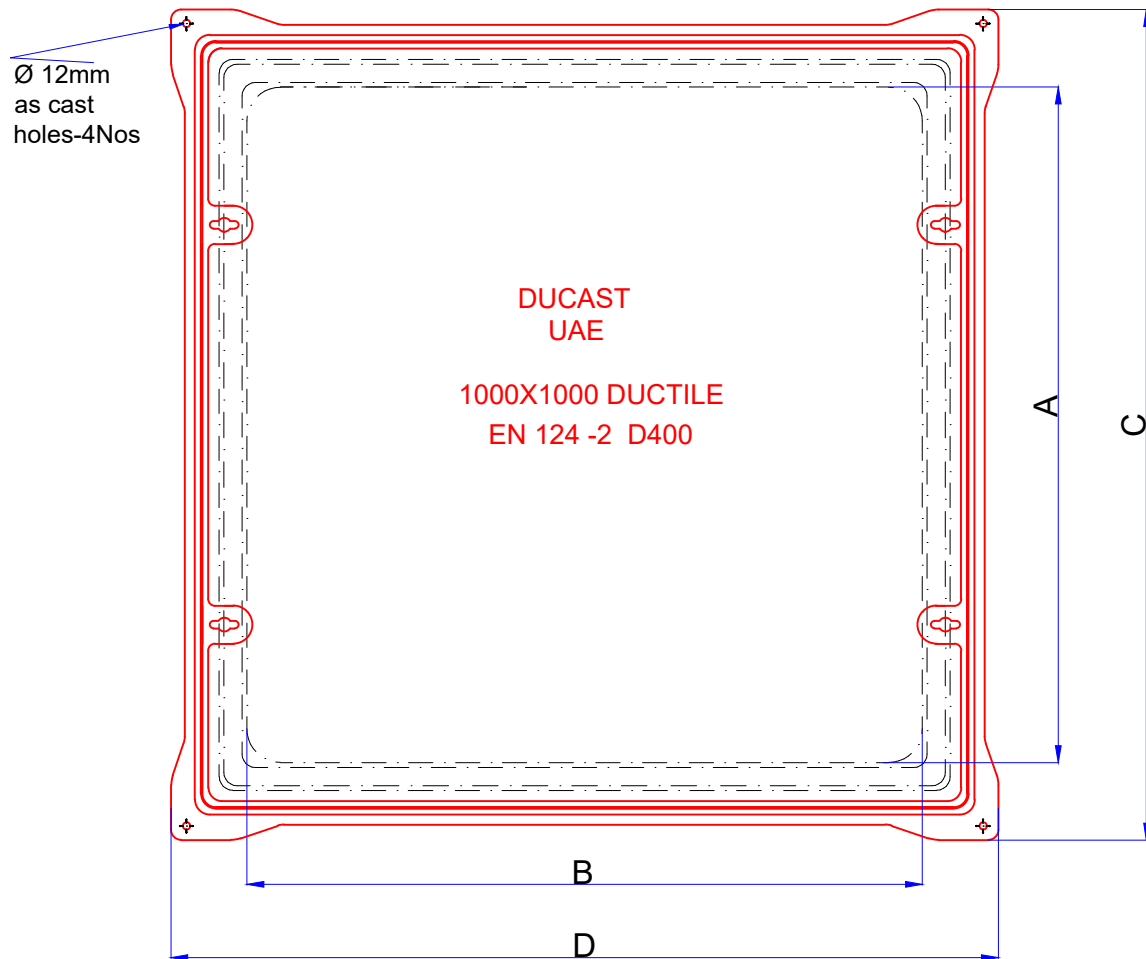
Plan View
