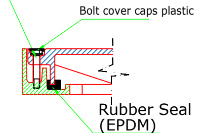
Sectional View -M Lockable Area
