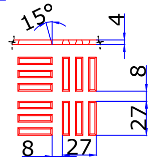
RAISED PATTERN DETAILS RAISED PATTERN THICKNESS 4.0MM
