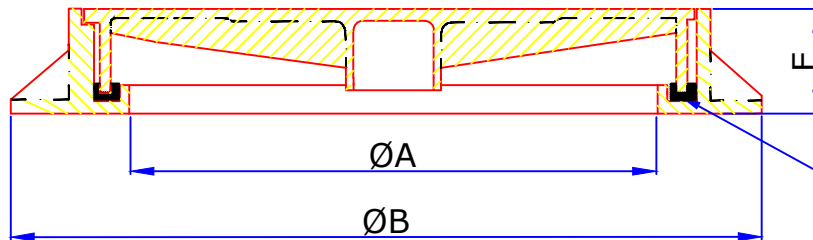
SECTIONAL VIEW
