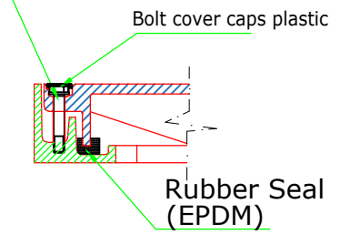
Sectional View -M Lockable Area
