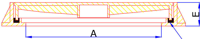
SECTIONAL VIEW OF COVER & FRAME
