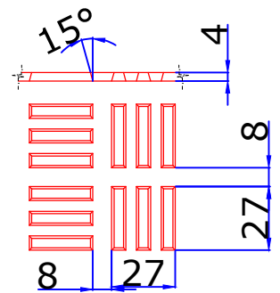
RAISED PATTERN DETAILS
