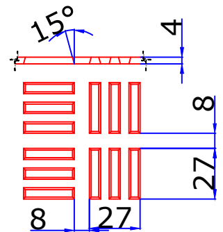
RAISED PATTERN DETAILS RAISED PATTERN THICKNESS 4.0MM
