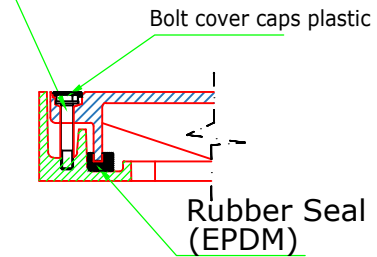
Sectional View -M Lockable Area
